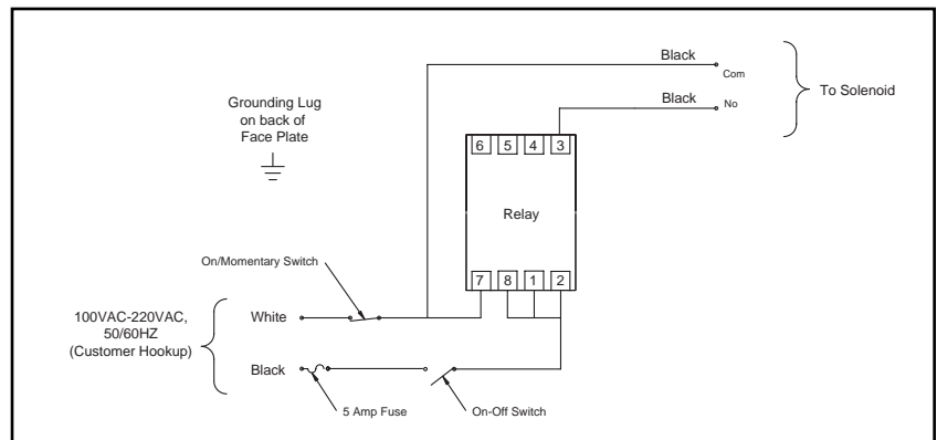
WIRING DIAGRAM
