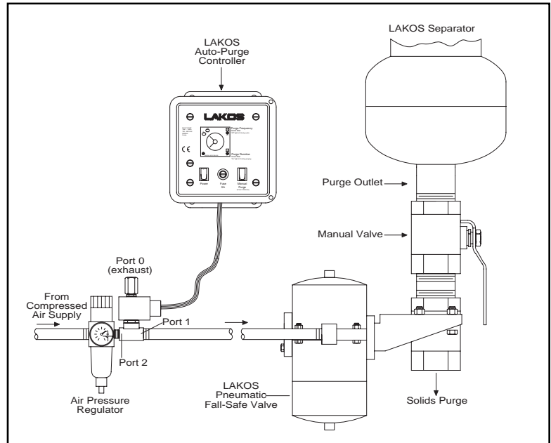
SUGGESTED INSTALLATION
